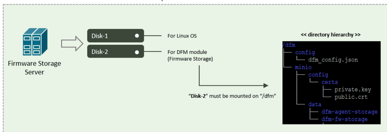
Fig 4-7 An Disk Partitions for DMF Module on Firmware Storage(minio) server
