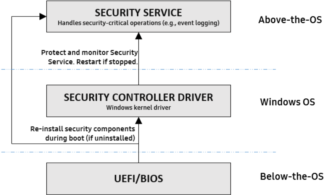
Figure 6: Samsung Security Service Tamper Protection from Below-the-OS
